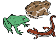
Amphibians
