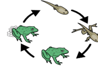
Life Cycle
